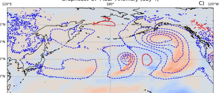
Graphcast-OP MSLP Anomaly (day 4)
